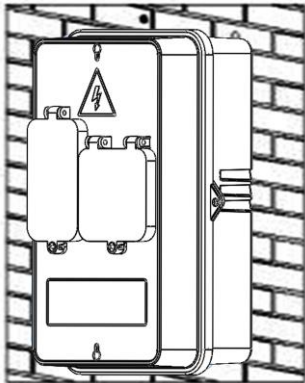
Wall installation
